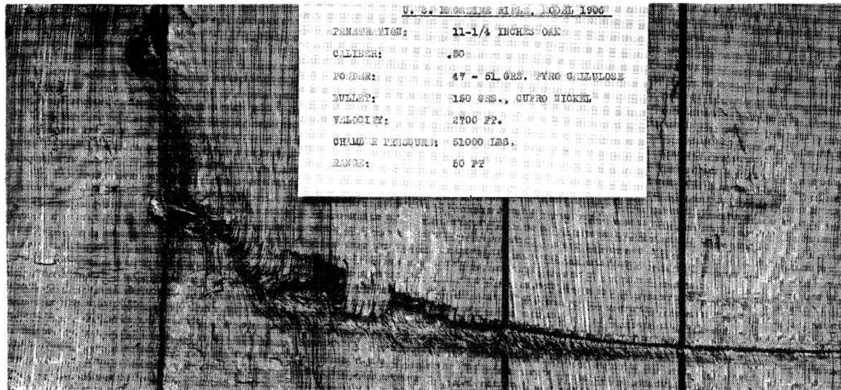
Penetration of 11 \frac{1}{4} inches in oak by .30-'06 150 grain bullet driven at 2700 f.s., range, 50 feet. The penetration is much less than that achieved at longer ranges. The reason is that at this short range, the bullet had not settled down to a stable flight, and when it encountered the resistance of the oak it yawed badly, and rapidly gave up all its energy.
