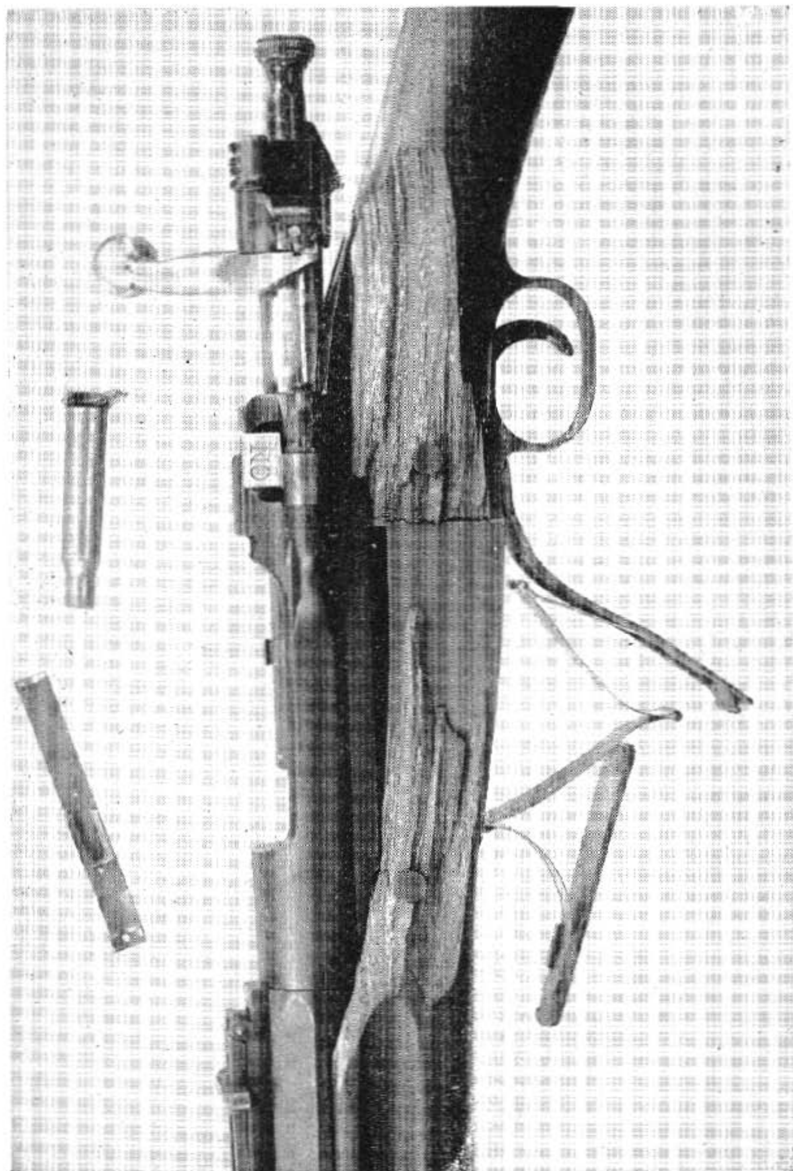
This double heat treated receiver and bolt withstood a destruction charge of 45 grains of bullseye behind a 170 grain flat based proof bullet, giving a pressure of around 133,000 pounds per square inch. The head of the case practically melted away, letting the gas out into the receiver well, where it messed things up a bit, and blew splinters off the stock, but the action held firm.
