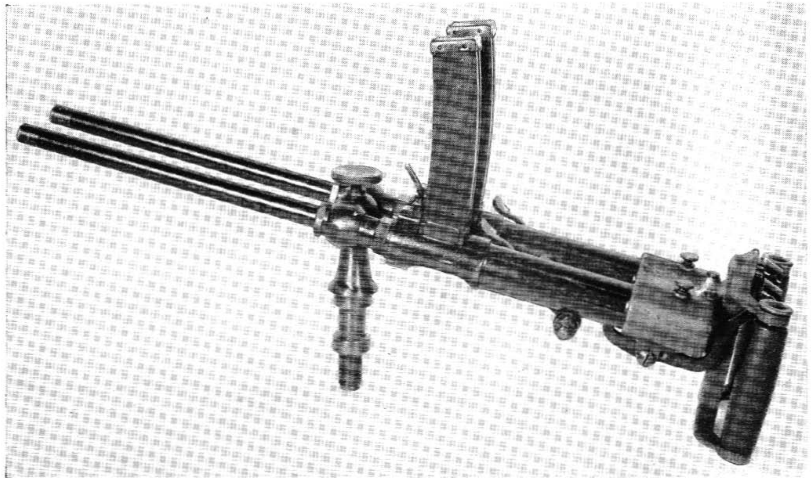
The first Submachine gun; the Italian Villar Perosa, shooting the 9 mm Parabellum (Luger) pistol cartridge. I tested this gun in 1917.
