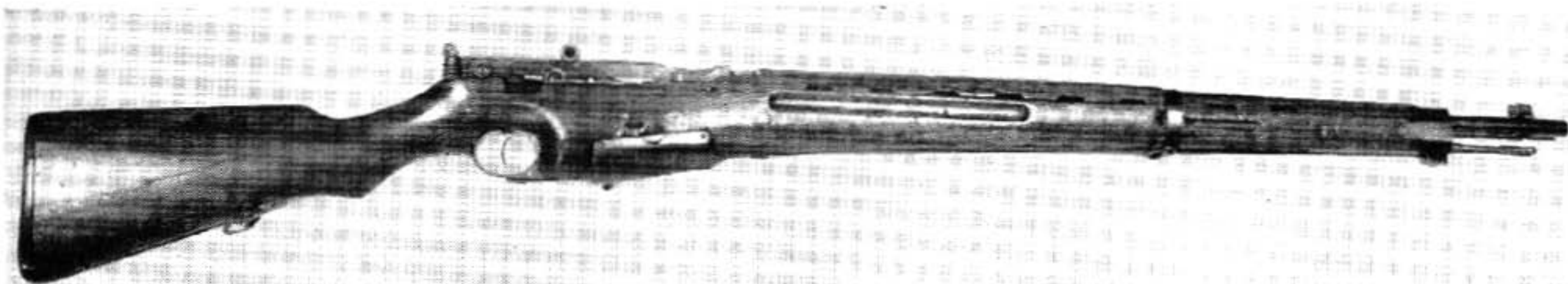
Japanese copy of the Pedersen semiautomatic rifle. Unlike the Pedersen, this rifle uses a rotary magazine similar to the Schoenauer type, or to that used in the Savage Model 1899, and is arranged to be loaded by stripping cartridges from a clip like that of the Springfield or Mauser.
