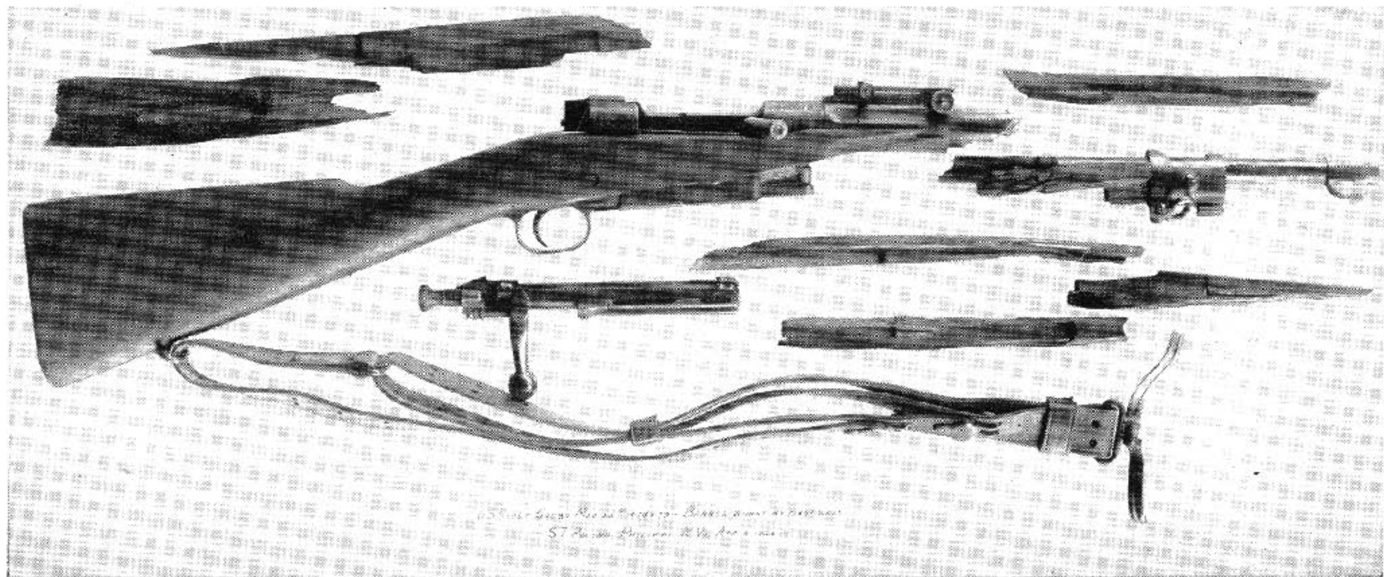
The barrel of this rifle burst on the first shot when the owner fired it with the barrel full of cosmoline. The low-numbered receiver No. 478,579 with its bolt, both of the old heat treatment, did not fail.
