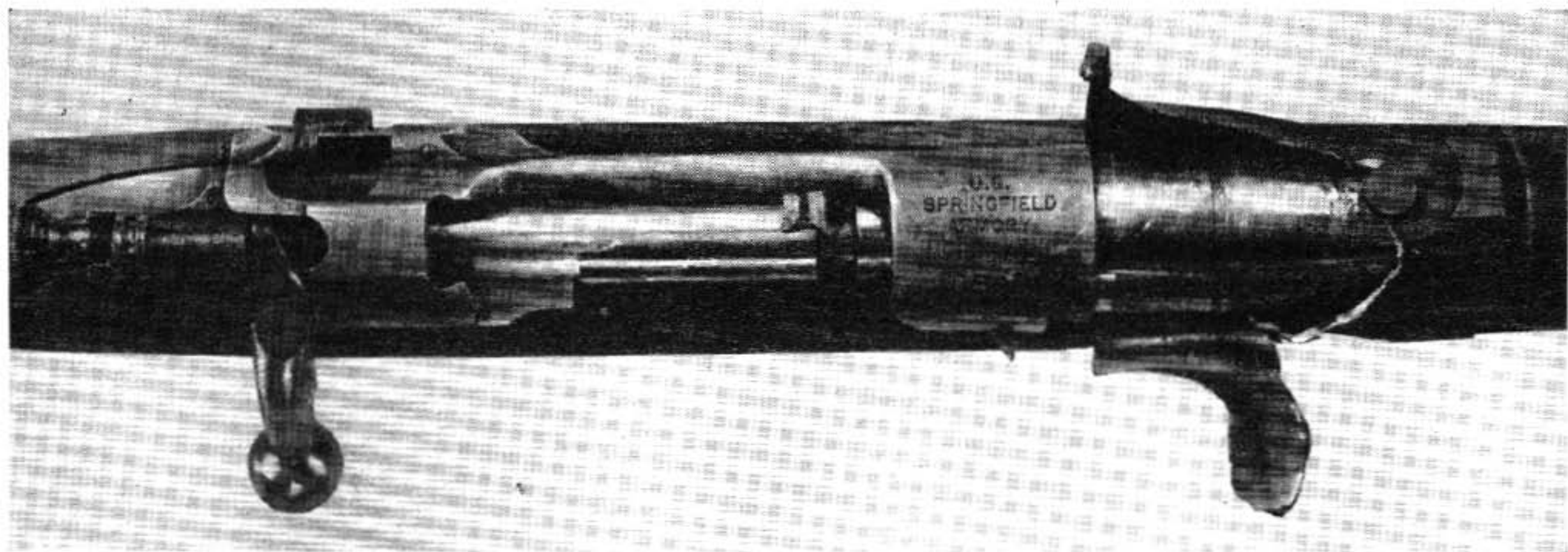
Result of a hidden seam in the barrel. After the adoption in 1918 of a double heat treatment for the receiver and bolt, it was the practice to select a rifle occasionally from production and subject it to the highest pressure that could be obtained in a test cartridge. This rifle, selected at random from production on May 3, 1918, was first tested with ten 70,000 pound test shots, then was fired with a 125,000 pound test cartridge. The receiver and bolt held, as they invariably did with this double heat treatment, but the hidden seam in the barrel opened up, with the results shown.
