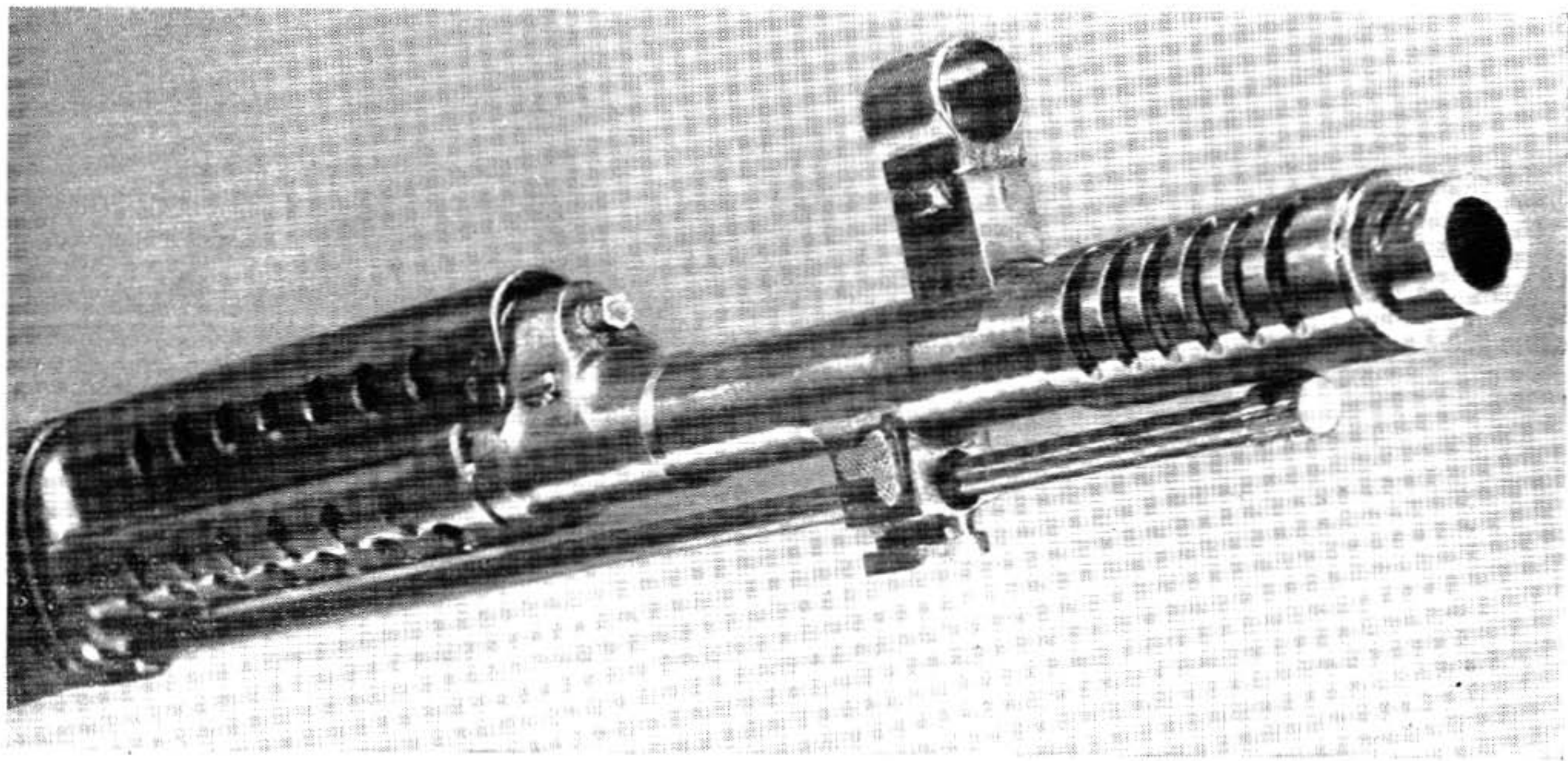
The muzzle brake on the Russian Tokarev semiautomatic rifle. This was widely used in World War II.
