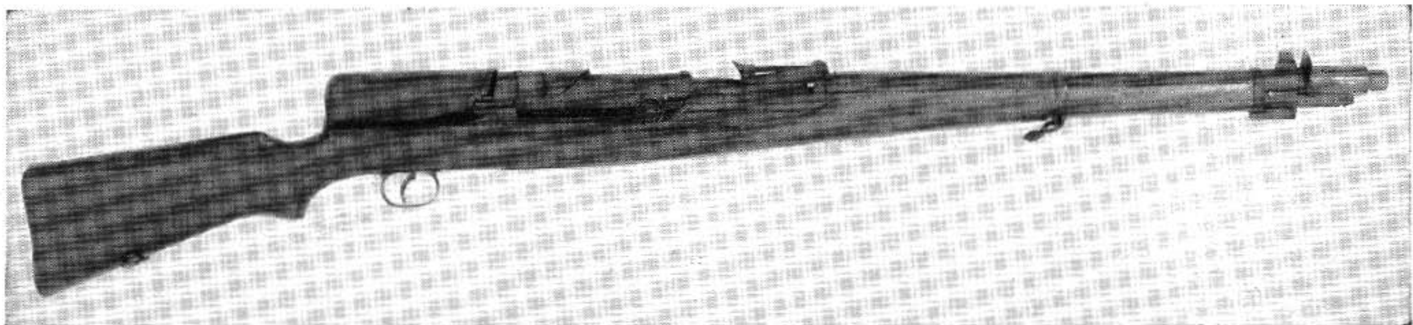
The Bang semiautomatic rifle, model of 1911. This gun is operated by the pull of the muzzle blast on a sliding cap over the muzzle. The pull is transmitted to a lever in the breech through a thin rod. This gun passed a most creditable test, but failed of adoption principally because the very thin barrel heated up too much in rapid fire. The gun is shown with a muzzle protector in place over the end of the barrel. It must be removed before firing.
