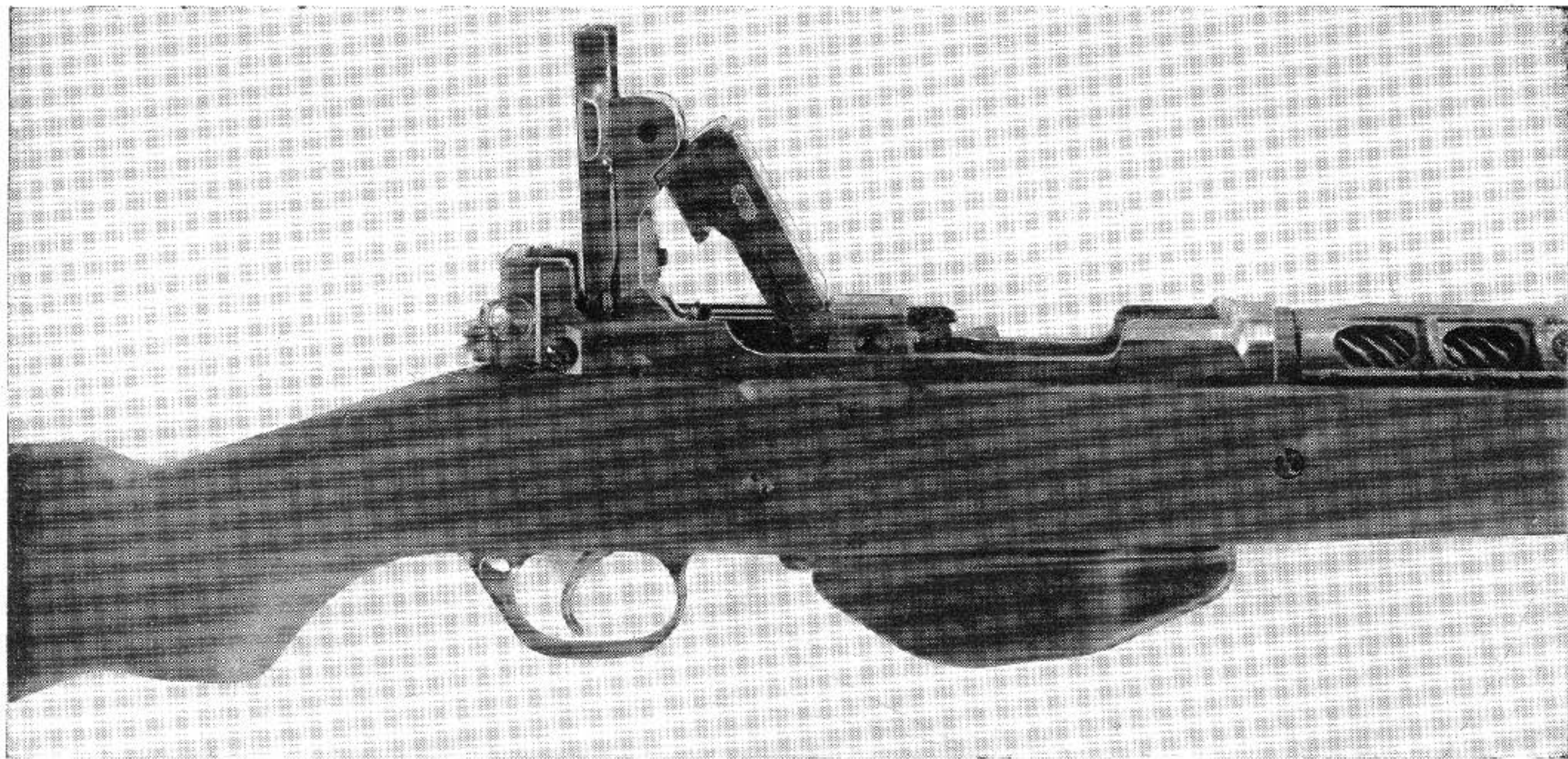
The Pedersen .276, shown with action open.
