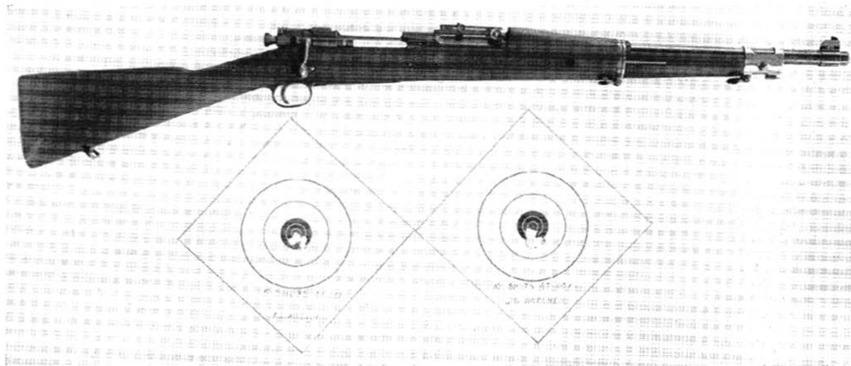
Experimental Carbine, shooting the .45 caliber service automatic pistol cartridge, made at Springfield in 1921. It had a 20 inch barrel.
