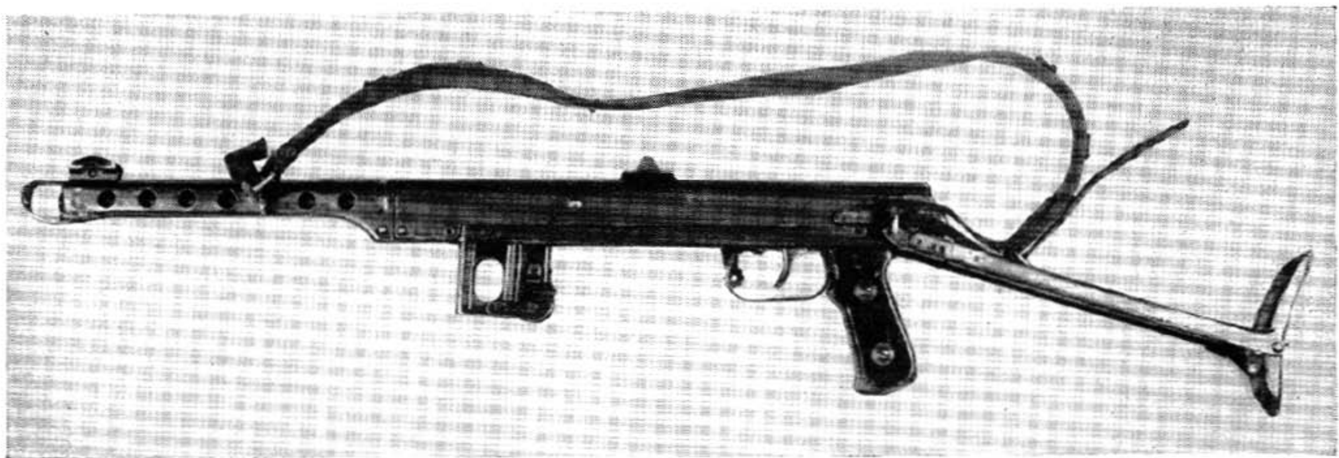
The Russian Sudiaev 7.62 mm machine pistol or submachine gun called PTS 1943.
