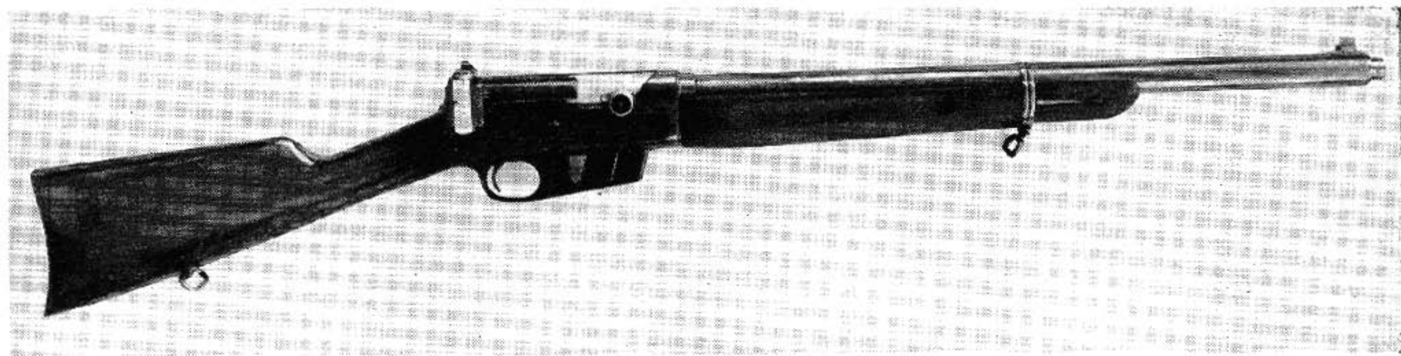
The Remington autoloading rifle, model 8 (now model 81) fitted for military use. During the years around 1930, when we were trying to find a suitable semiautomatic rifle for adoption, a number of these Remingtons, in .35 caliber were fitted up like this and issued to the Army for tactical tests to determine the best way to use a semiautomatic rifle in various situations.
