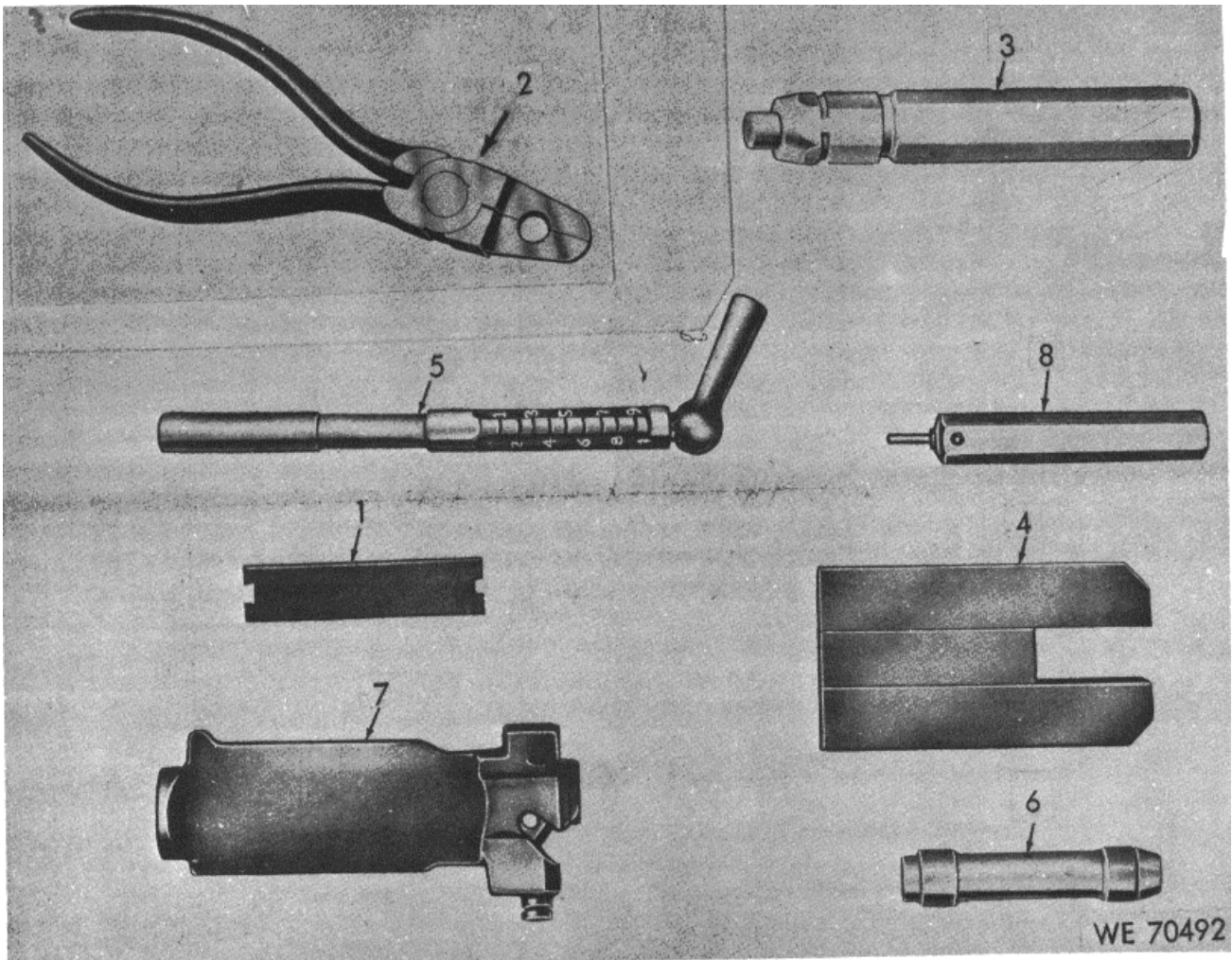
Figure 15. Maintenance Tools.
