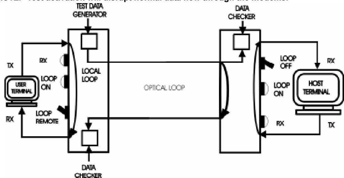
Figure 5-1. System Test Example From User-End of Fiber Link
