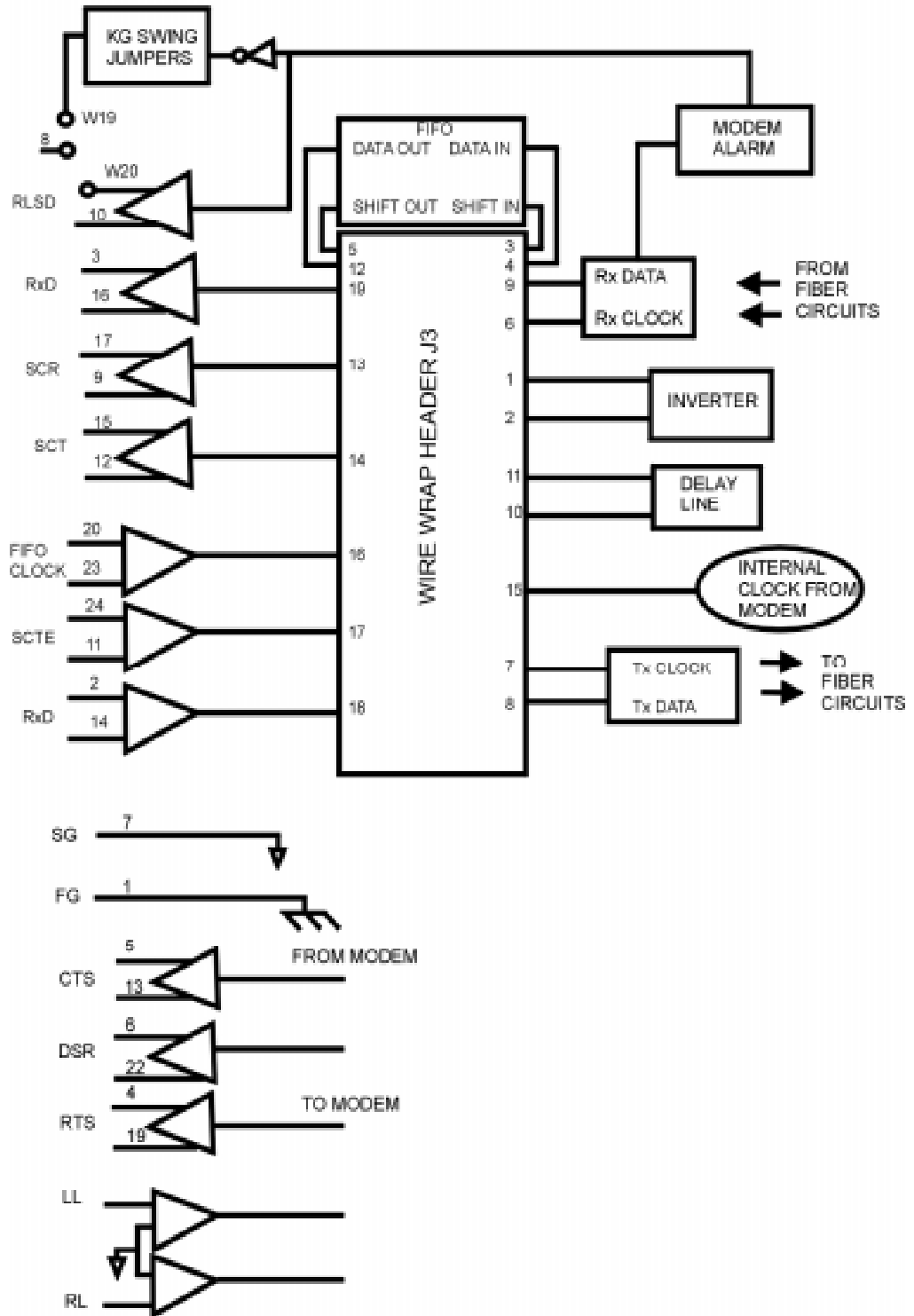
Figure 3-3. Available Strapping Options for Programmable Buffered Interface
