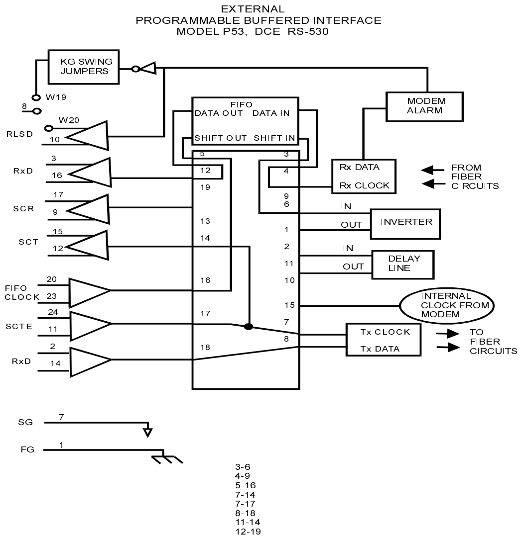
Figure 3-8. External Programmable Buffered Interface, Model P53
