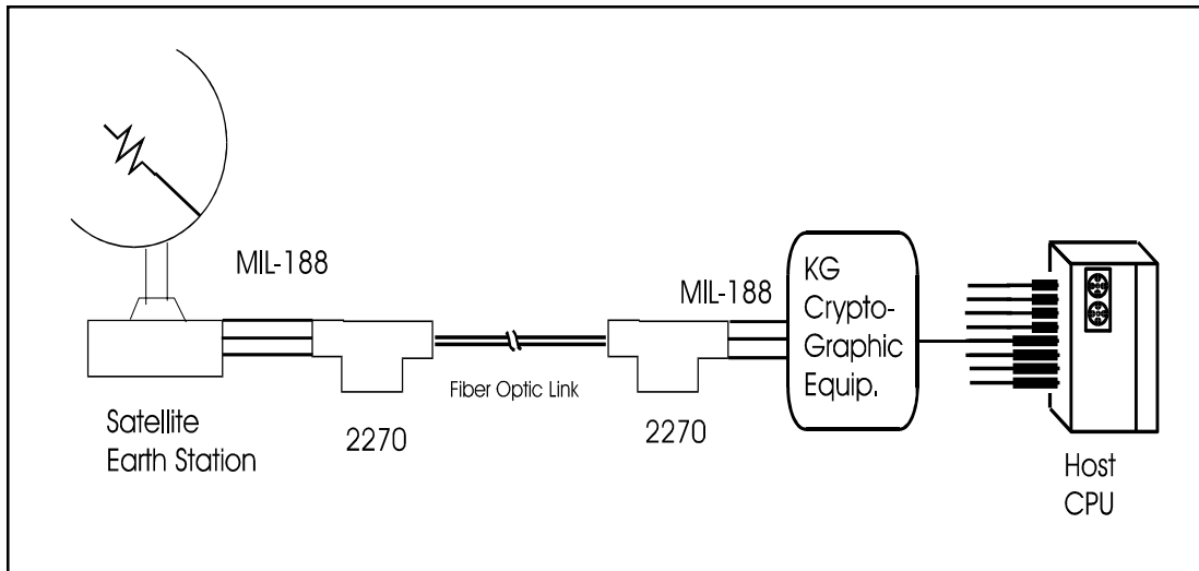
Figure 4-2. Typical High Speed 2270 Modem Application
