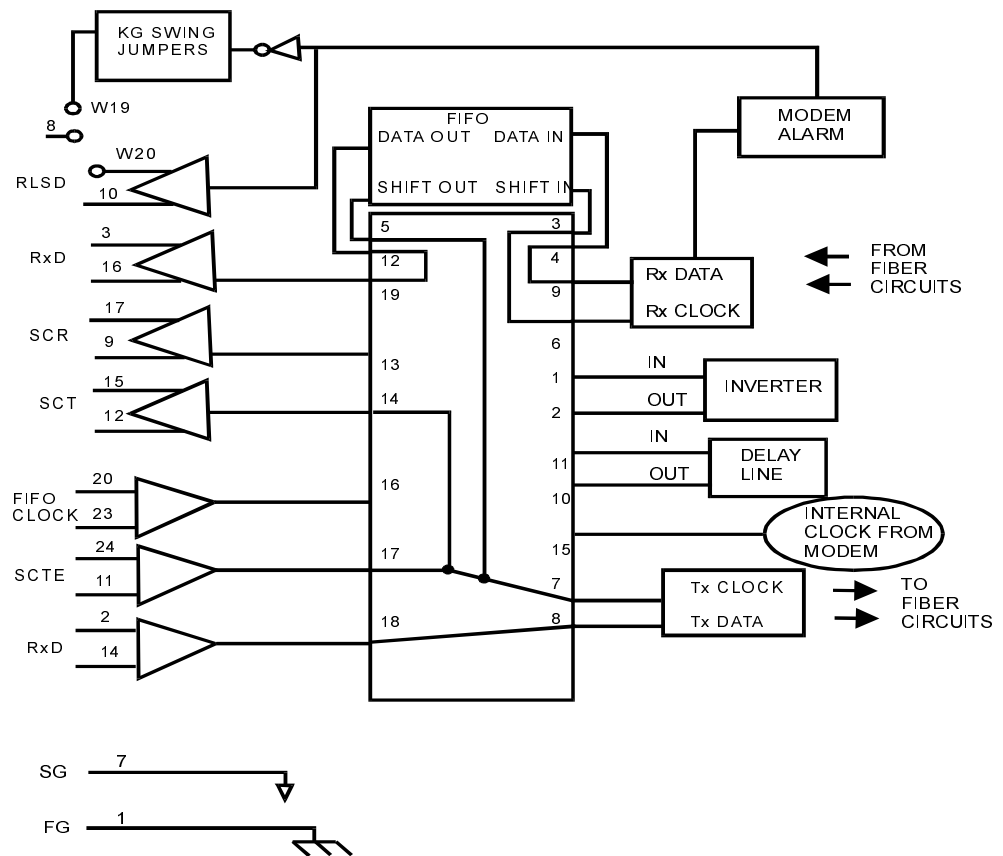
EXTERNAL STATION PROGRAMMABLE BUFFERED INTERFACE MODEL P53, DCE RS-530
