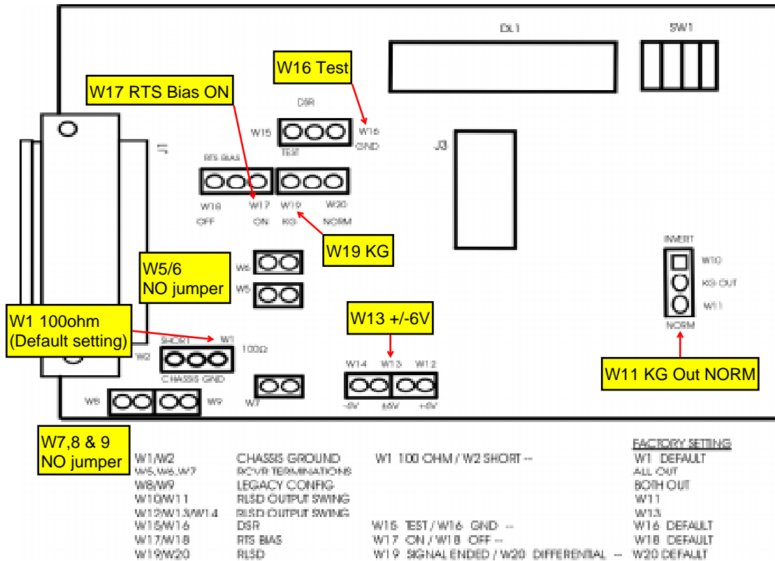
Figure 3-4. Board Layout for Programmable Buffered Interface
