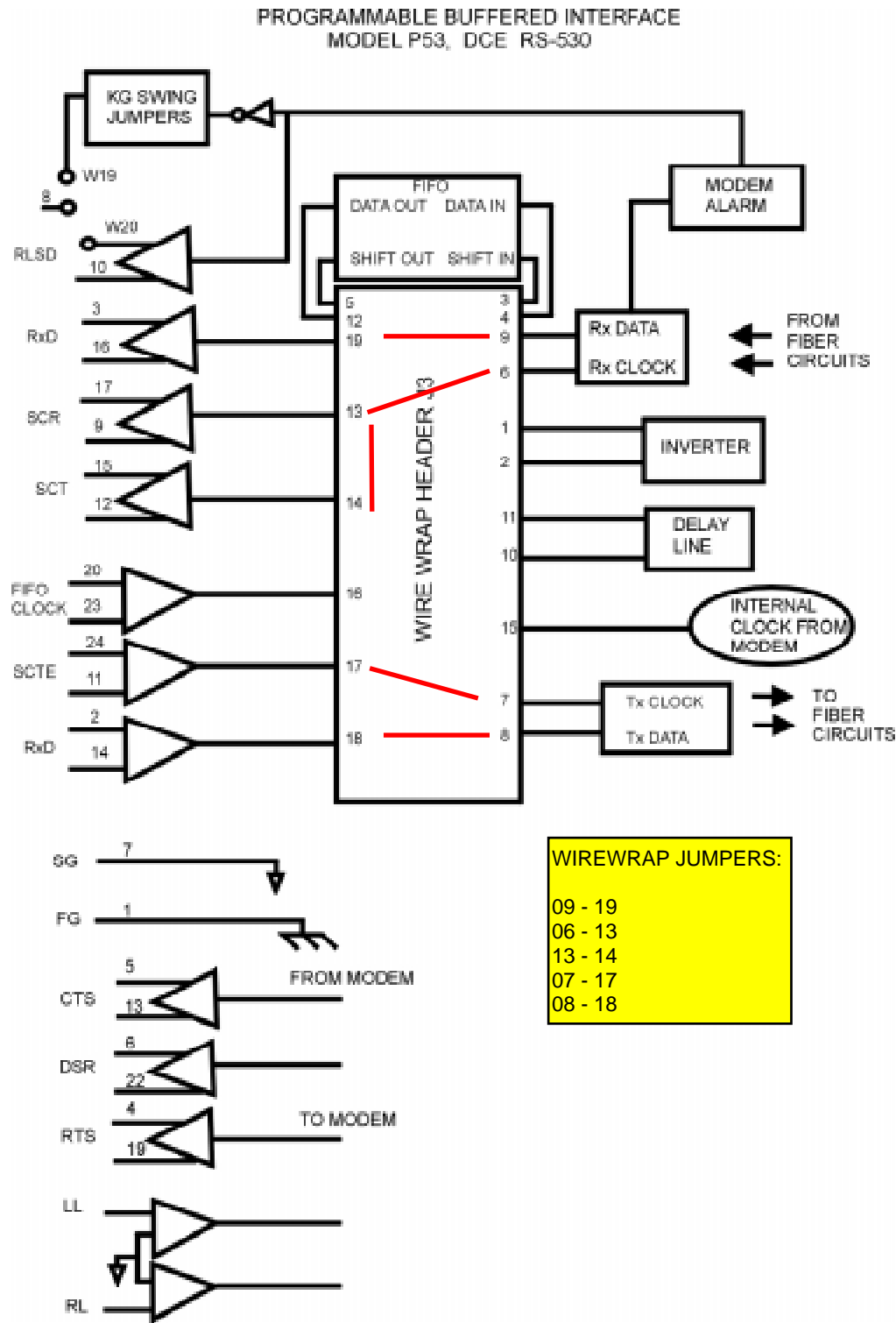
Figure 3-5. Programmable Buffered Interface, Model P53, DCE RS-530
