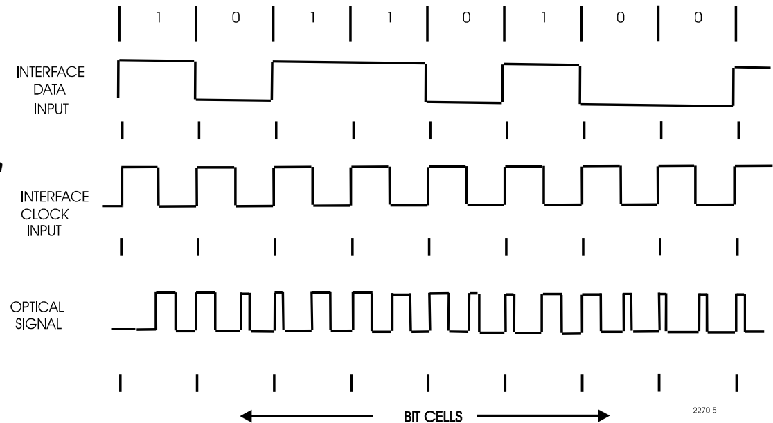
Figure 4-3. Data Organization with PWM Optics
