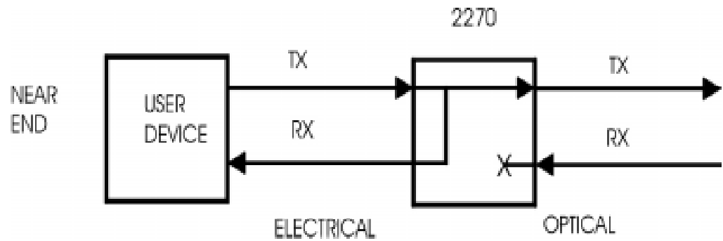
Figure 5-3. "Interface Only" Local Loopback Active
