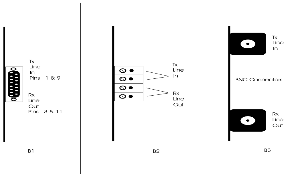
Figure 3-2. Transparent Bipolar Interface Connectors
