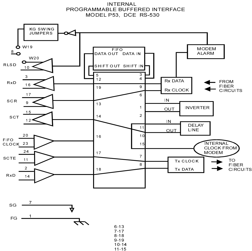
Figure 3-7. Internal Programmable Buffered Interface, Model P53, DCE RS-530
