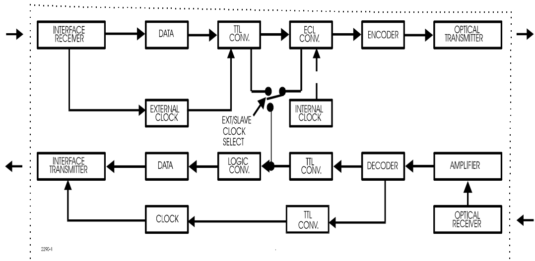
Figure 4-1. 2270 Circuit Board Diagram
