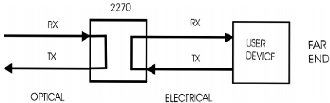
Figure 5-5. “Bi-Directional” Remote Loopback Active
