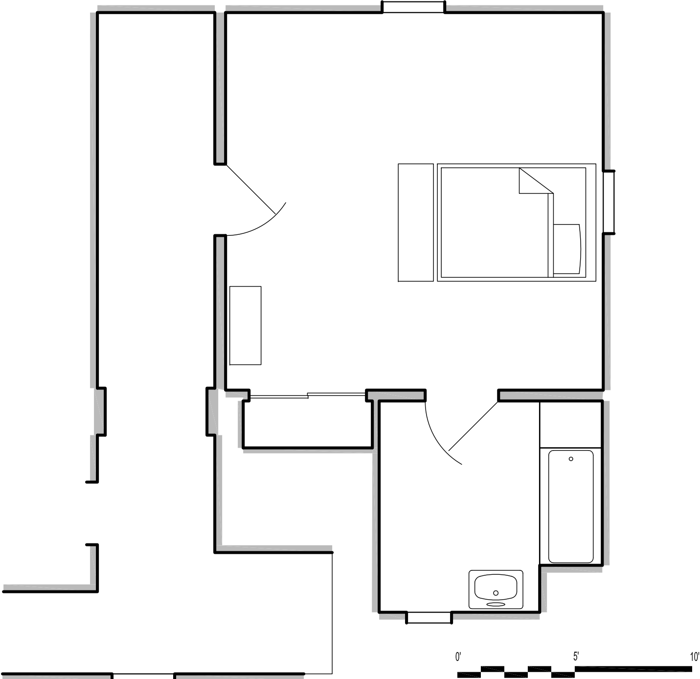
SCOTT'S BEDROOM INTERIOR - DIRECTOR'S PLAN - NORTH STAGE - SCALE: 1/4" = 1'-0" - 5-11-16
