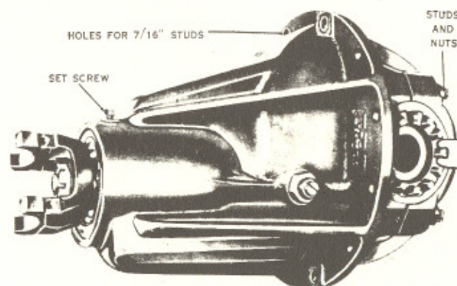
Figure 5-4 -- 9-5/8 Ring Gear and Carrier Assembly
